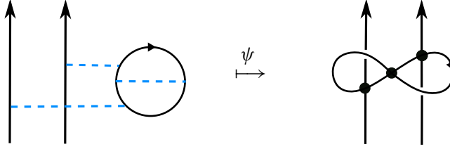
Figure 16. Example of \psi with the right-hand side viewed as an element of \tilde{\mathcal{T}}_3/\tilde{\mathcal{T}}_4 . Different choices of over- or under-crossings with the poles only differ by elements of \tilde{\mathcal{T}}_4 .
