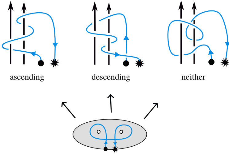
Figure 27. A curve in \mathbb{C}\pi lifted to ascending, descending, and neither ascending nor descending bottom tangles. The three tangles are equivalent in \tilde{\mathcal{T}}^{1/1} , but distinct in \tilde{\mathcal{T}} .
