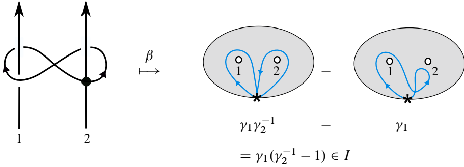
Figure 21. Example calculation demonstrating that \beta is a filtered map.
