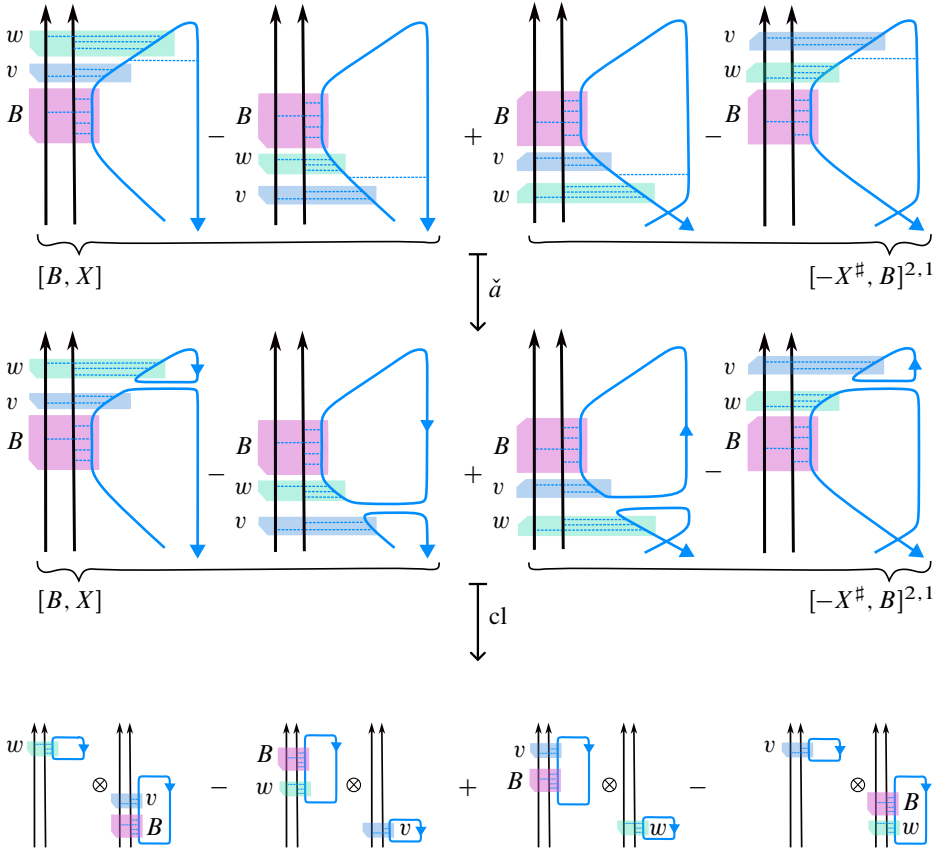
Figure 38. Calculation of the term in \varepsilon_1(D) corresponding to X .
