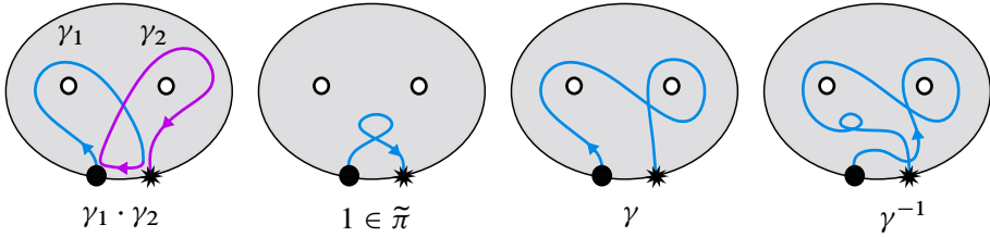
Figure 5. The group structure on \tilde{\pi} .
