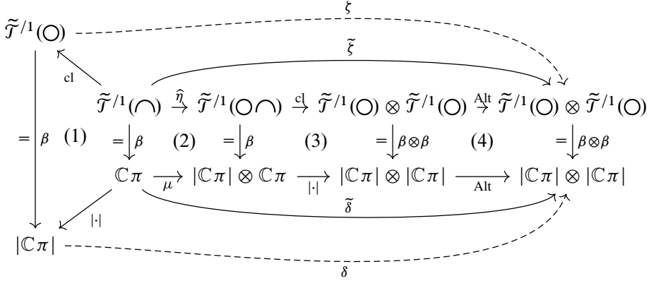
Figure 32. The map \zeta realises the Turaev cobracket \delta .
