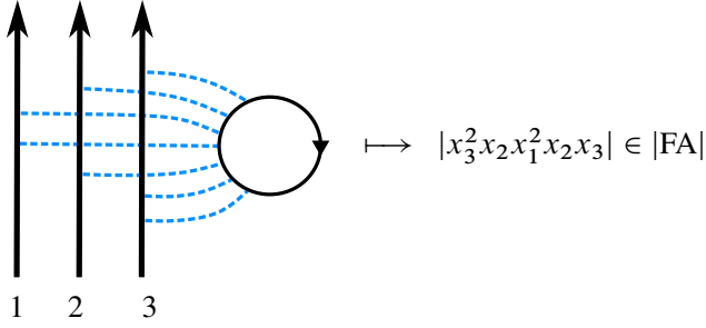
Figure 22. An example demonstrating how chord diagrams with no strand-strand chords can be read as cyclic words in |FA| .
