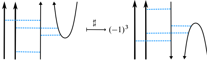
Figure 18. An example chord diagram and its flip.
