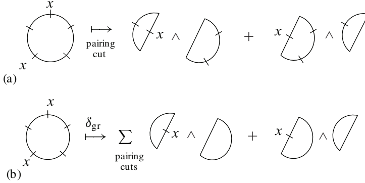
Figure 9. (a) An example of a pairing cut of a cyclic word. (b) An example of the graded Turaev cobracket as a sum over pairing cuts of a cyclic word.
