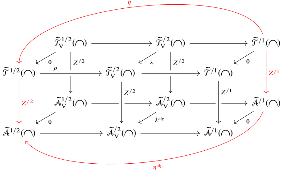
Figure 36. Commutative cube showing the compatibility of \eta and \eta^{\text{alg}} with the Kontsevich integral.
