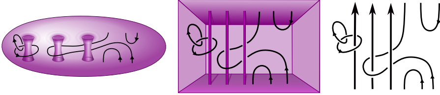
Figure 10. An example of a tangle in M_3 , drawn first in a handlebody, then in a cube with poles, and lastly as a tangle diagram projected to the back wall of the cube.
