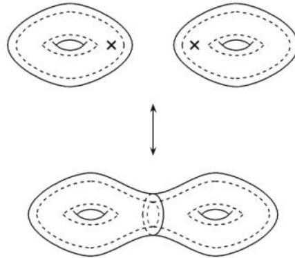
Figure 1: The stabilization move on S \times I .
